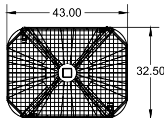
CHANGE-OUT RACK
